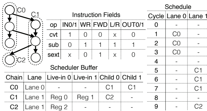
Figure 8: Example DFG execution on Chainsaw .
